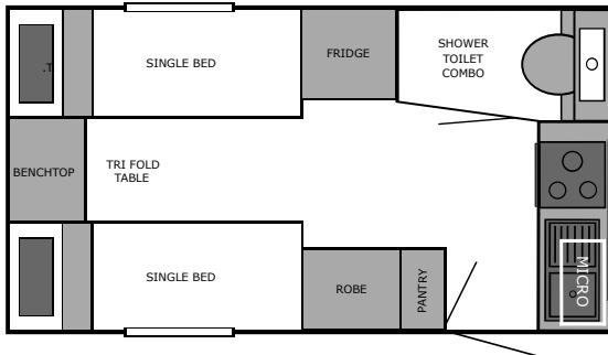
13'X7'-2 SPRINTER
